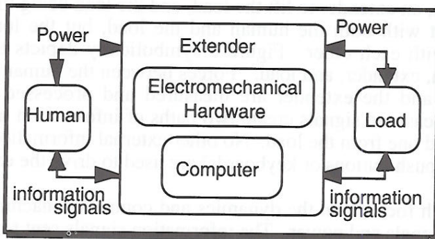
Figure 2: The extender motion is a function of the forces from the load and the human, in addition to the command signal from the computer.
