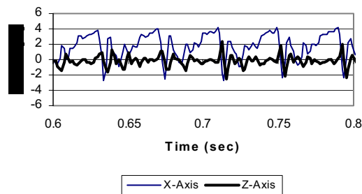
Figure 7. Force measurements in time domain when moving across the upper portion of 3D square-wave gratings
