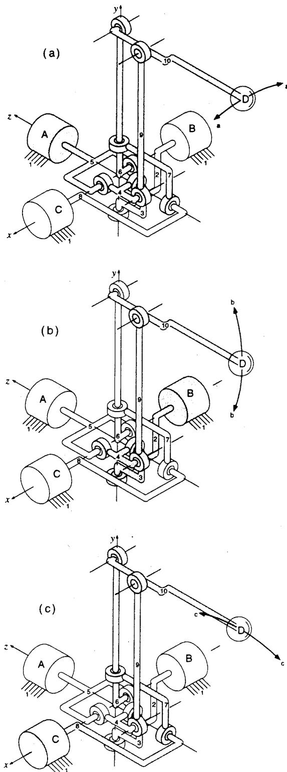
Figure 1. 10 Link 12R mechanism with different actuators enabled.
