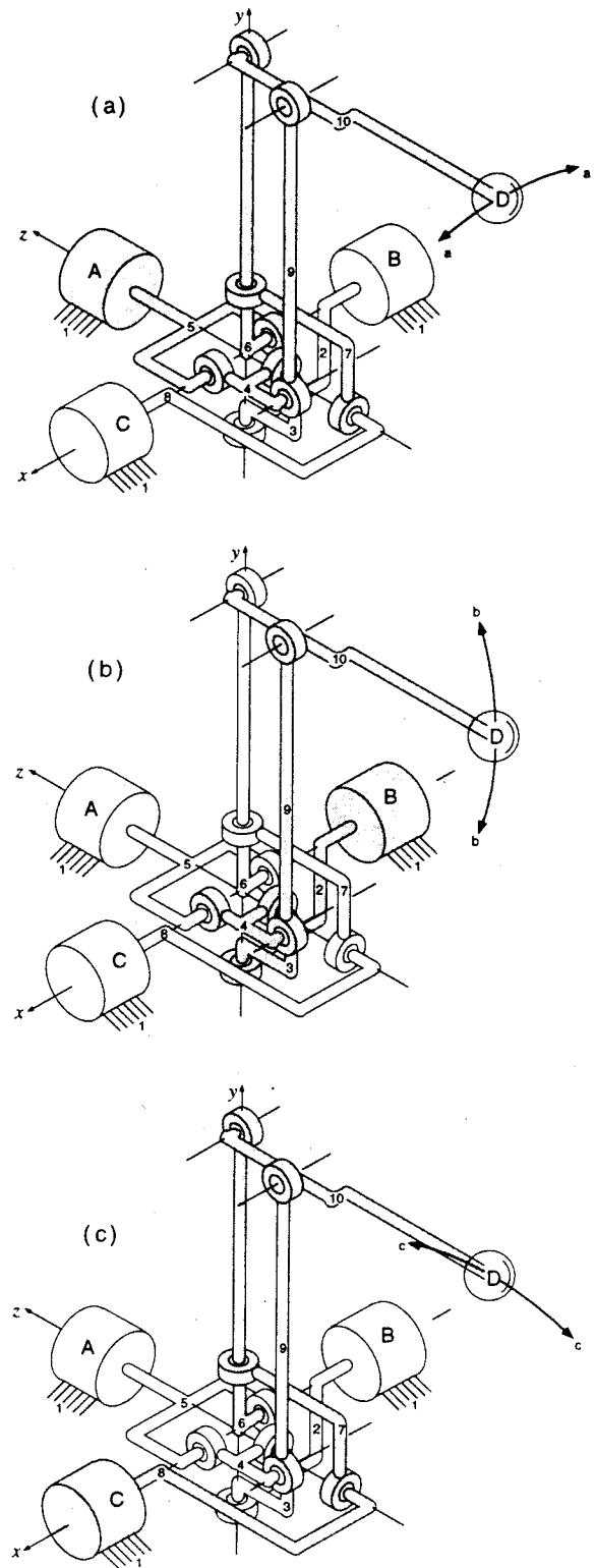
Figure 1. 10 Link 12R mechanism with different actuators enabled.
