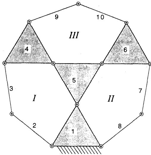
Figure 2. Planar equivalent 10 Link 12R mechanism.
