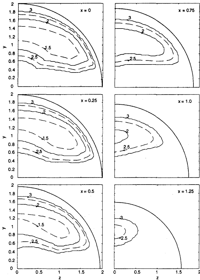
Figure 5. Condition number c(\mathbf{J}^T) for 10 Link 12R mechanism for slices x = 0.0, 0.25, 0.5, 0.75, 1.0, and 1.25 . The heavy gauge arc corresponds to the maximum reach in the respective x plane. Note that the quarter plane y, z \geq 0 in each slice is symmetric about both y and z axes.
